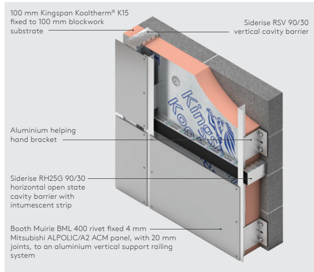
Figure 6: A2 ACM & Masonry Blockwork
