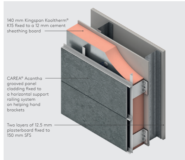
Figure 10: Acantha Grooved Panel & SFS
