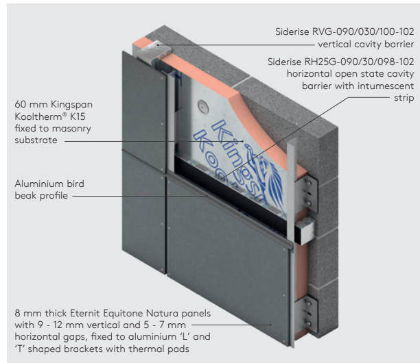
Figure 14: Fibre Cement Panels & Masonry Blockwork
