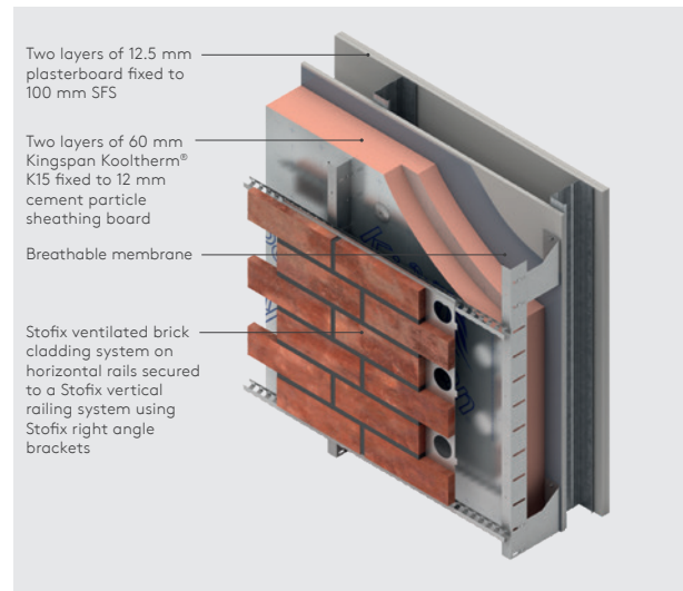
Figure 11: Ventilated Brick Cladding System & SFS
