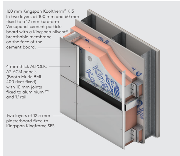
Figure 14: A2 ACM & Kingspan Kingframe SFS
