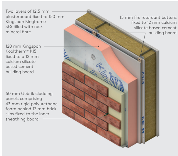
Figure 12: Gebrük Cladding Panel & Kingspan Kingframe SFS Filled with Rock Mineral Fibre
